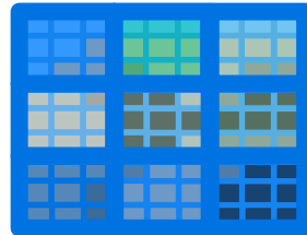
Weather Vector
