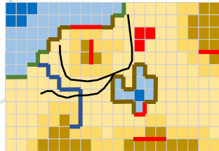
Terrain Vector
